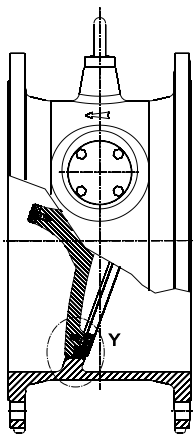
FIG. 1 Closed Position
