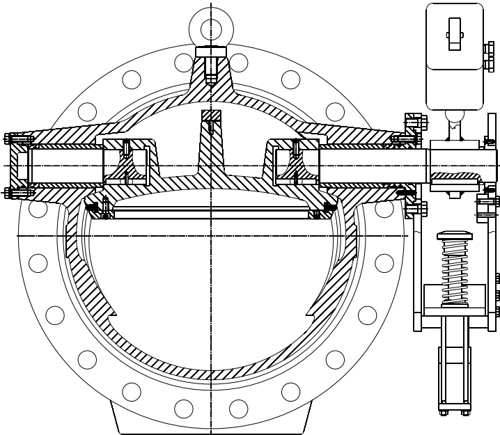
FIG. 8 Opened Position
