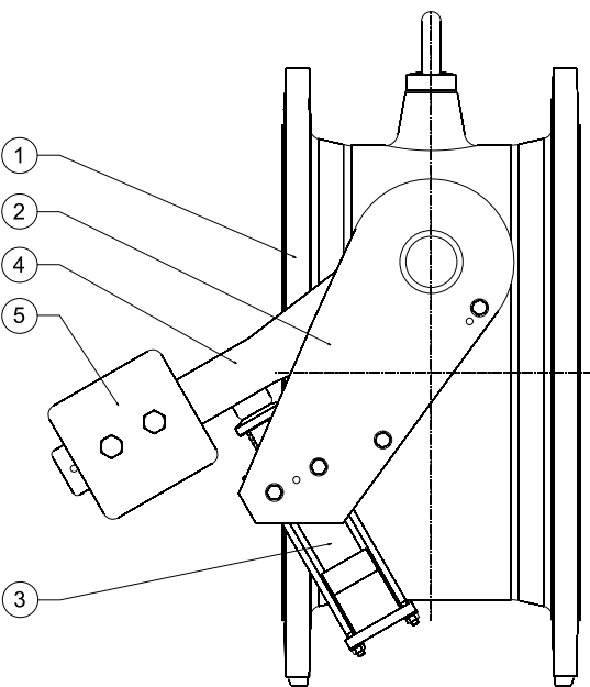
FIG. 7 Closed Position
