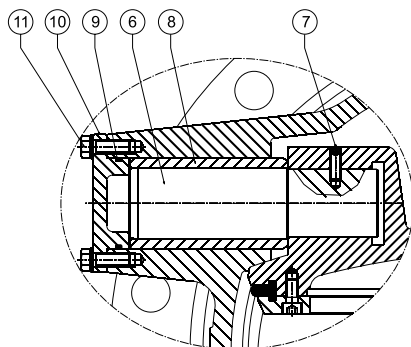
FIG. 4 Detail X
